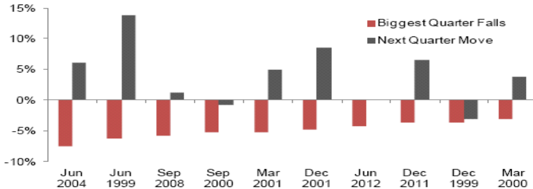
Fig. 1: Quarters when gold has fallen significantly, largely followed by positive quarters
